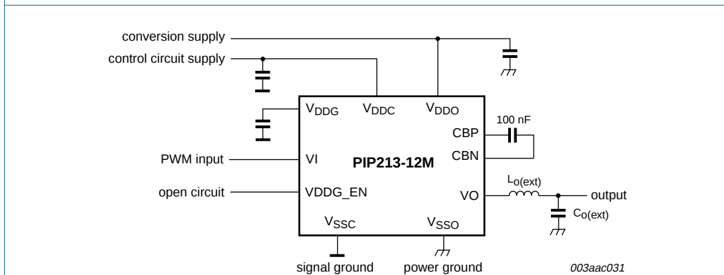
Fig 12. Single supply operation using internal supply for V_{DDG}
