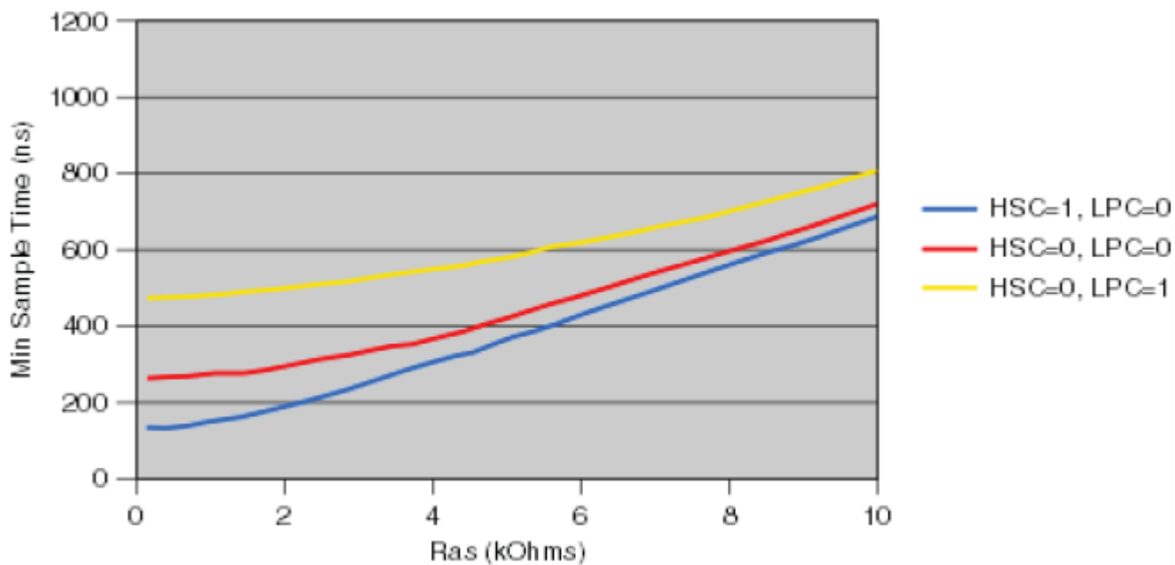
Figure 4-85. Minimum Sample Time Vs R_{\text{as}} ( C_{\text{as}} = 2\text{pF} )
