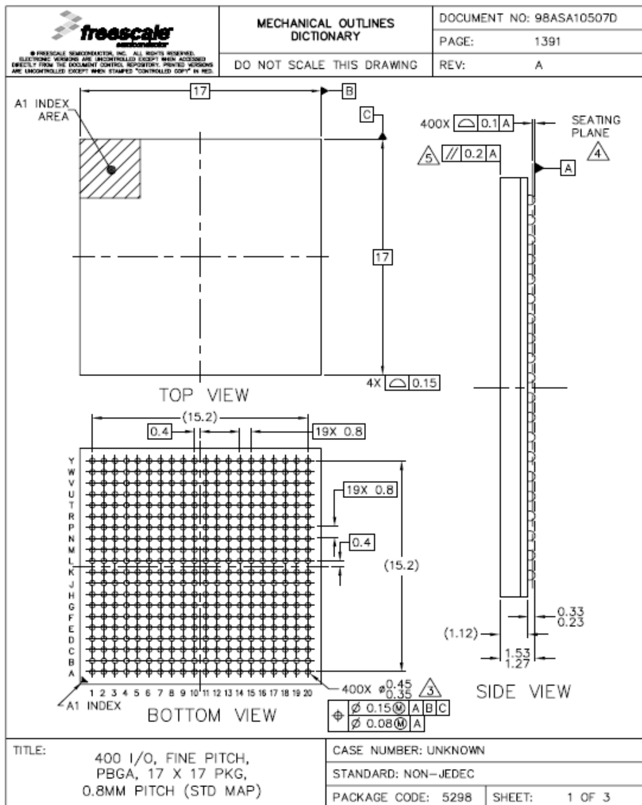
Figure 91. 17x17 mm BGA, Case x Package Top, Bottom, and Side Views
