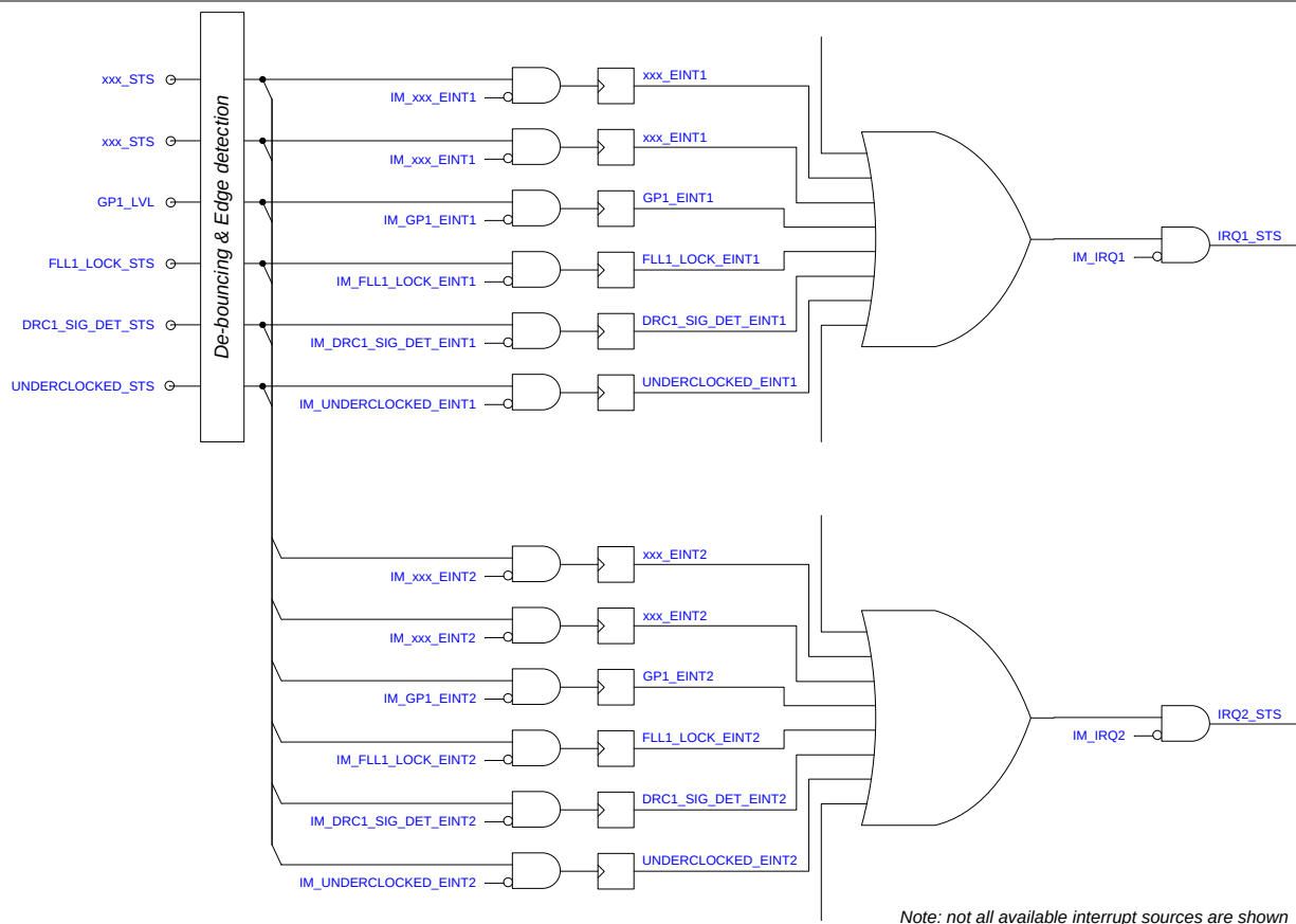
Figure 68 Interrupt Controller
