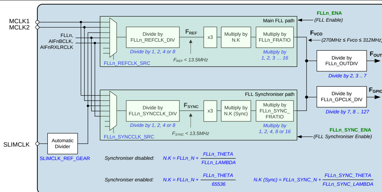
Figure 71 FLL Configuration
