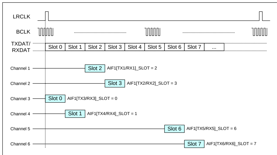
Figure 50 DSP Mode B Example
