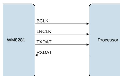
Figure 43 Master Mode
