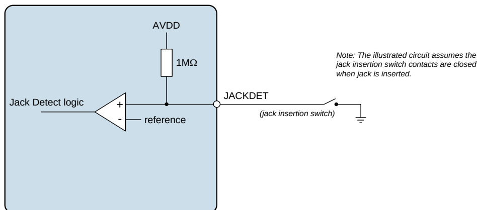
Figure 62 Jack Detect Comparator
