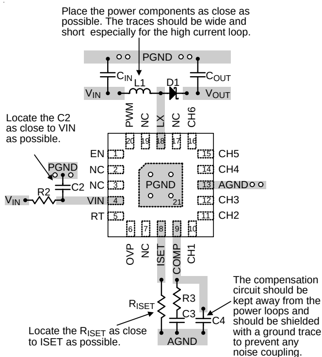
Figure 3. PCB Layout Guide
