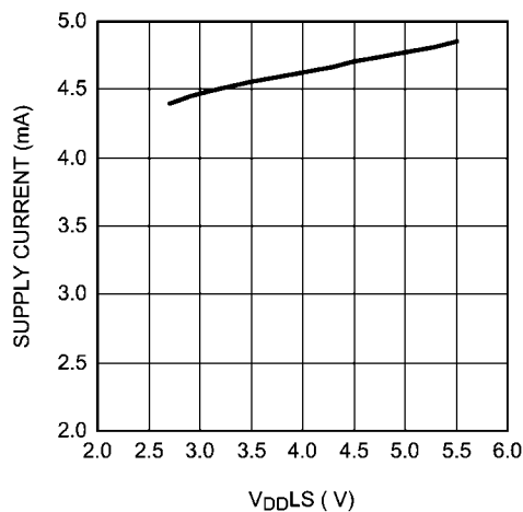
Supply Current vs V_{DDLS} V_{DDHP} = 2.8V , Mode 7, 10, 14, No Load
