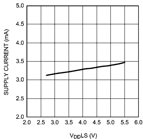
Supply Current vs V_{DDLS} V_{DDHP} = 2.8V , Mode 2, 4, 6, No Load
