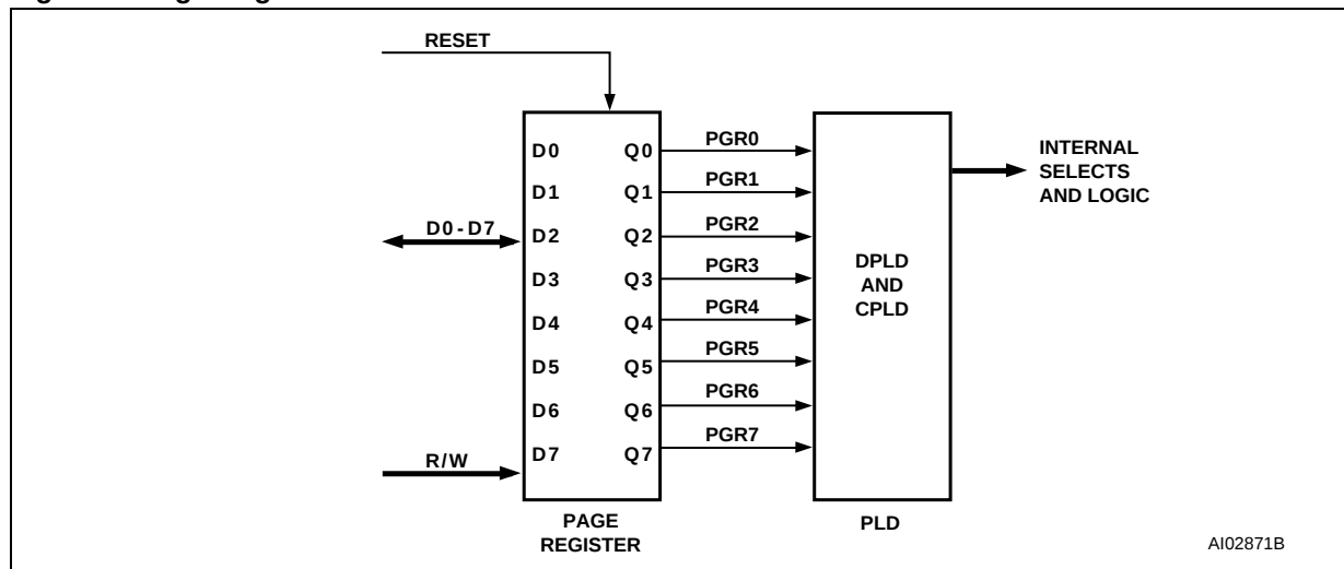
Figure 9. Page Register
