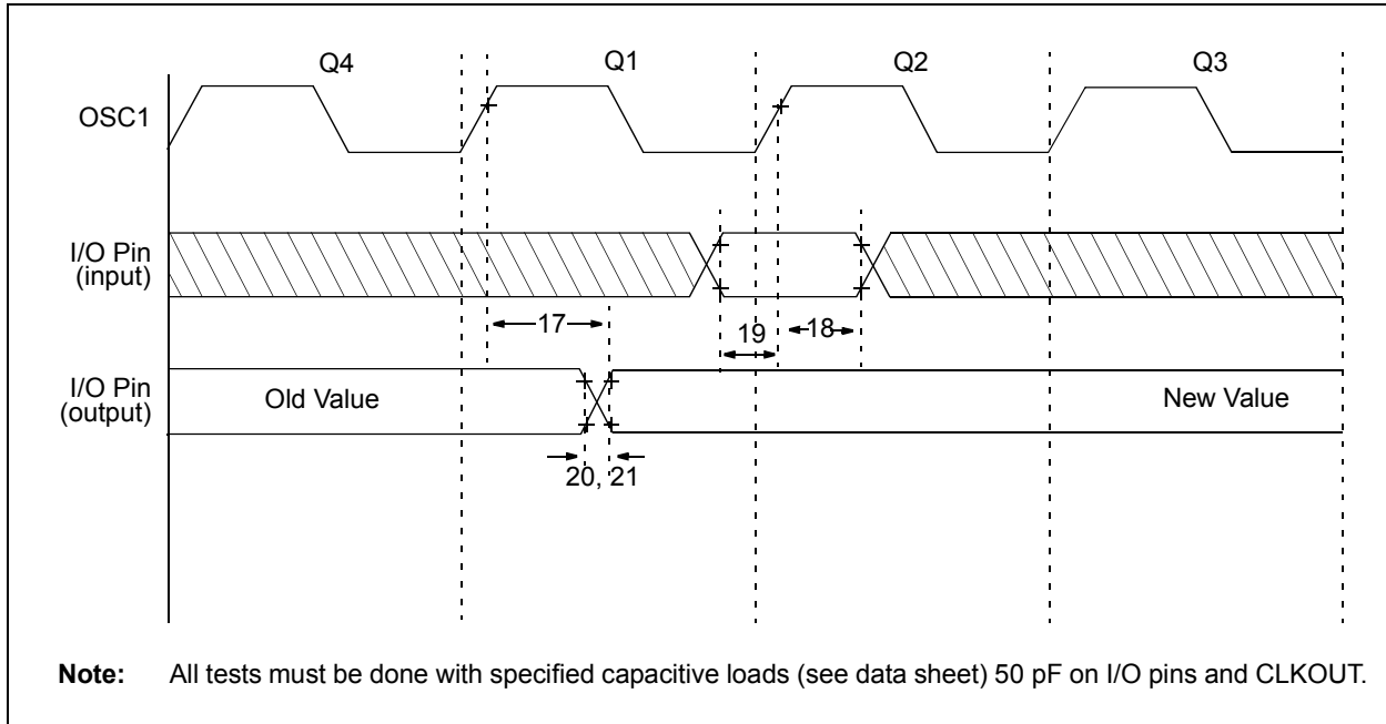
FIGURE 14-5: I/O TIMING
