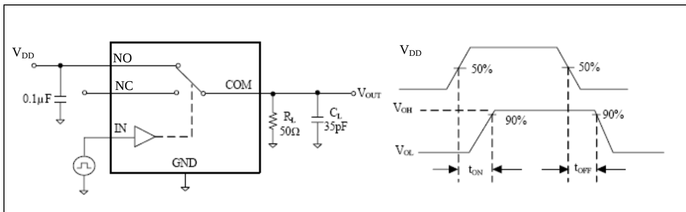
Figure 2. Switching Times
