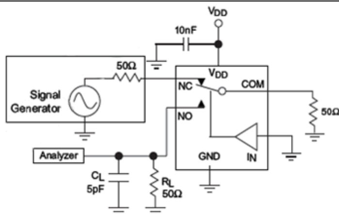
Figure 5. NC-NO Isolation
