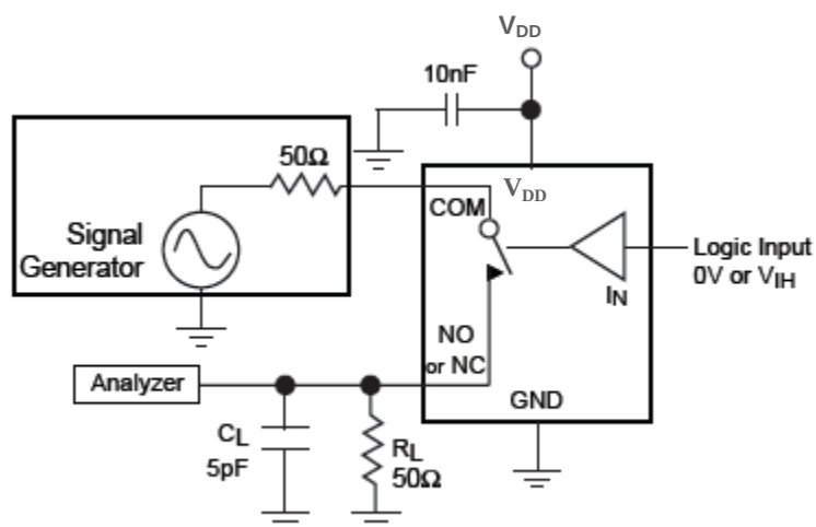
Figure 4. COM-NC/NO Isolation
