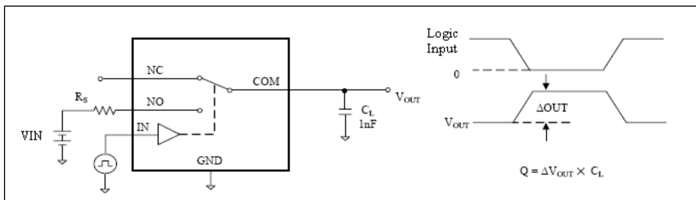
Figure 8. Charge Injection
