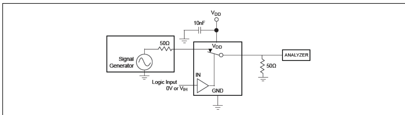
Figure 7. Bandwidth
