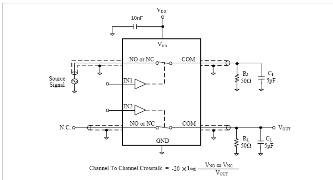
Figure 6. Channel-to-Channel Crosstalk
