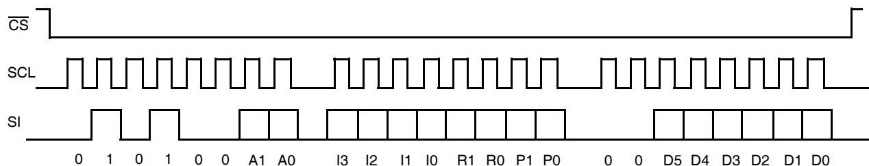
Figure 5. Three-Byte Command Sequence (Write)
