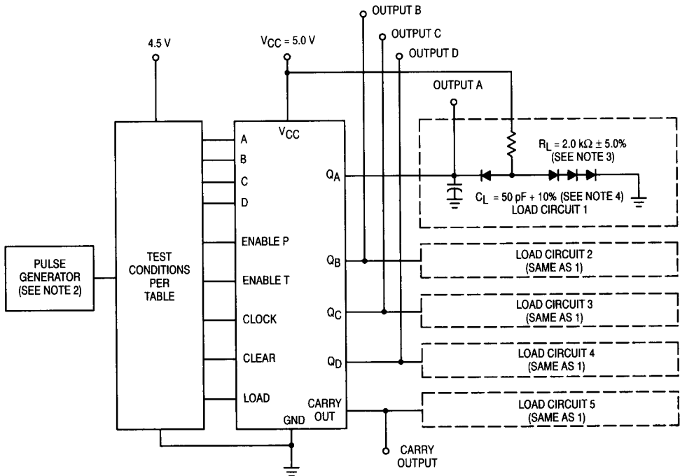
TEST CIRCUIT
