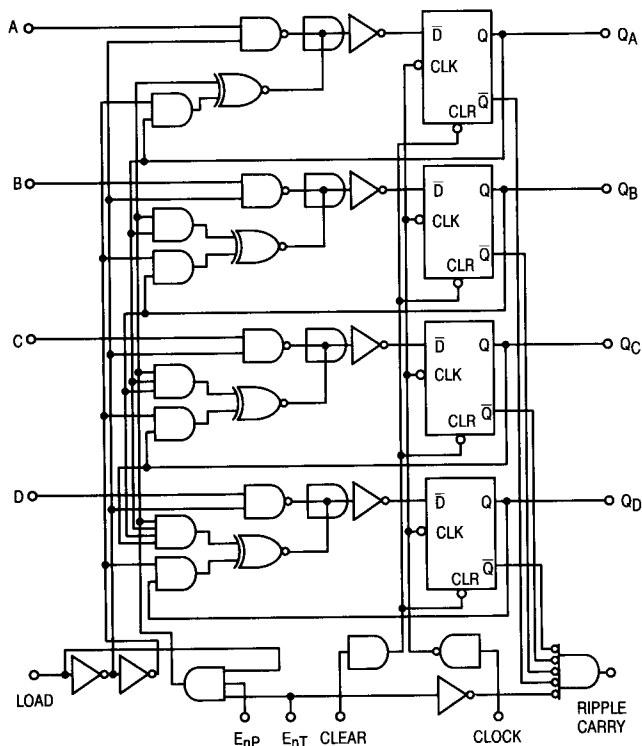
LOGIC DIAGRAM
