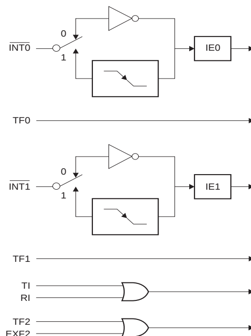
Figure 7. Interrupt Sources
