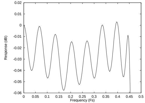
Figure 35 DAC Digital Filter Ripple – Type 1
