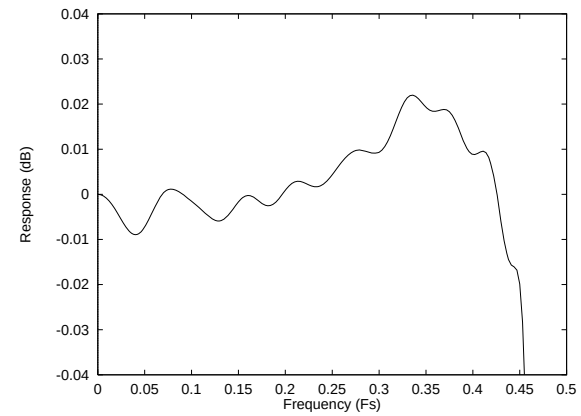
Figure 41 ADC Digital Filter Ripple – Type 0
