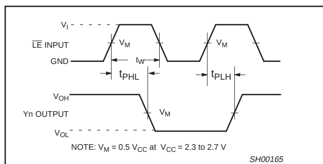
Waveform 2. Latch enable input ( \overline{\text{LE}} ) pulse width, the latch enable input to output ( \text{Y}_n ) propagation delays.
