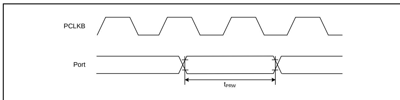
Figure 2.23 I/O Port Input Timing
