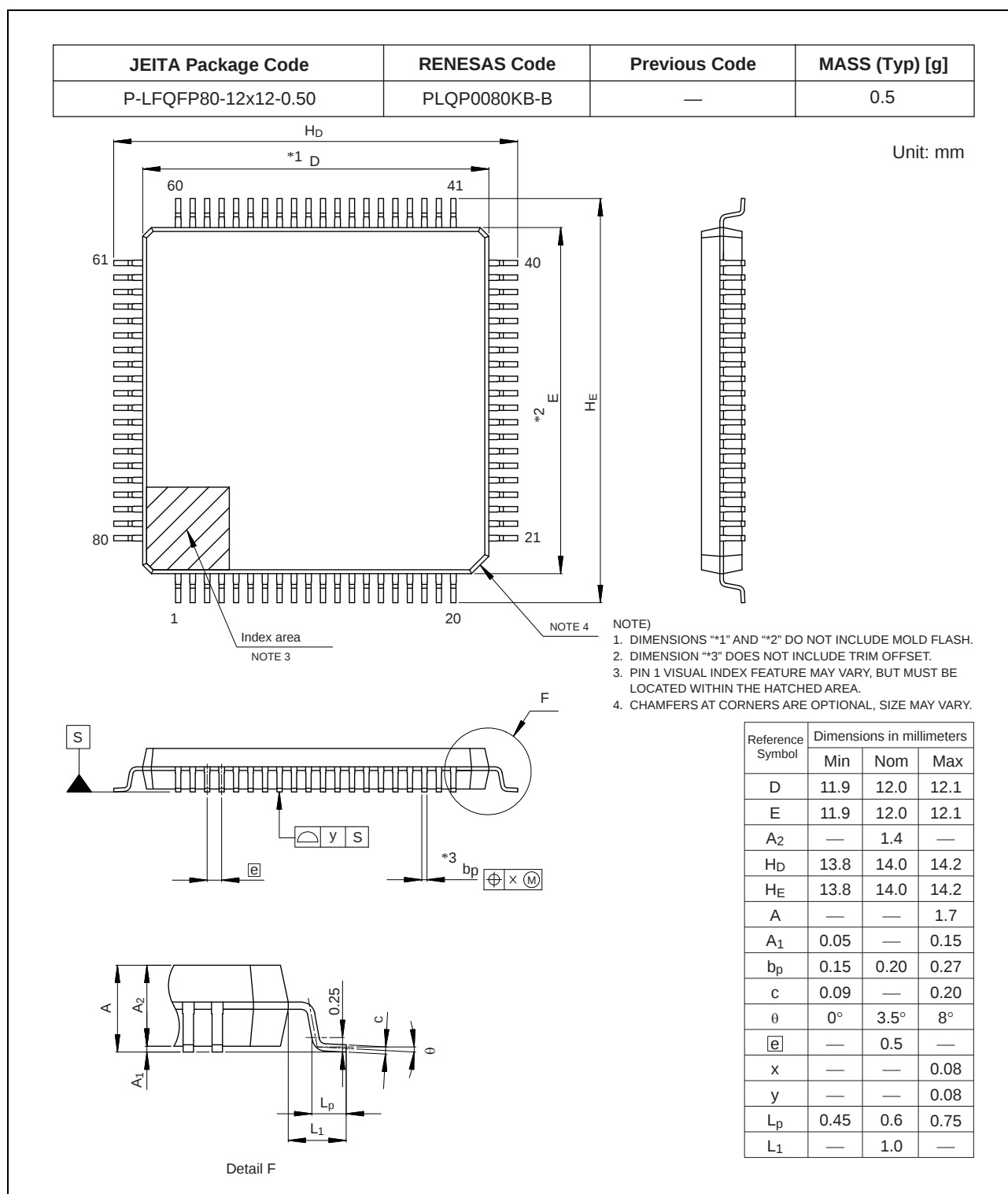
Figure E 80-Pin LFQFP (PLQP0080KB-B)
