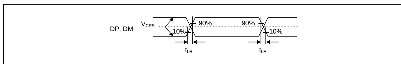
Figure 2.61 DP and DM Output Timing (Low Speed)
