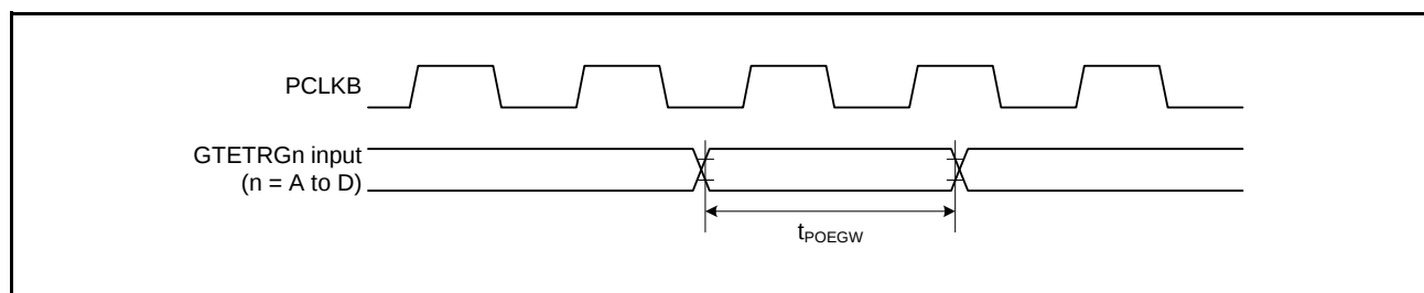
Figure 2.33 POEG Input Timing
