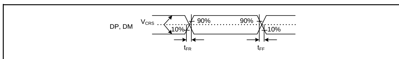
Figure 2.63 DP and DM Output Timing (Full-Speed)
