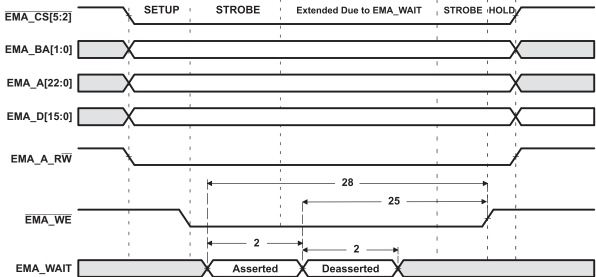
Figure 5-17. EMA_WAIT Write Timing Requirements
