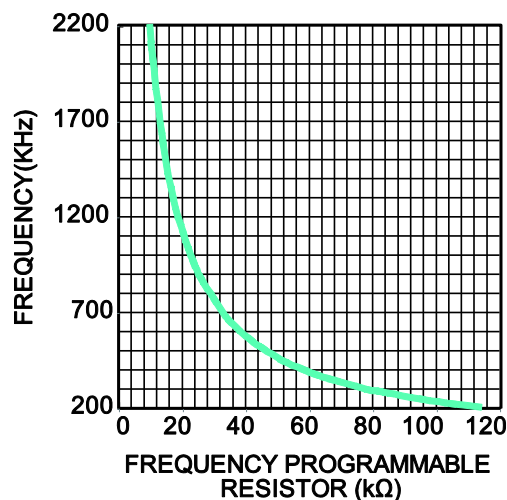
Figure 3: Switching Frequency vs. R_{FREQ}
