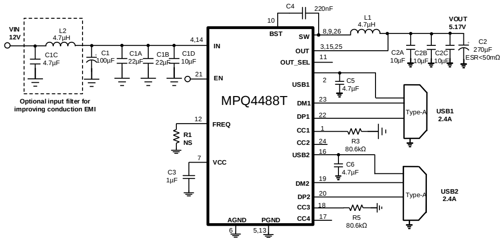
Figure 14: Dual USB Type-A 5V/2.4A Ports (13)
