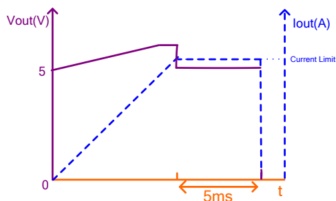
Figure 7: Over-Current Limit
