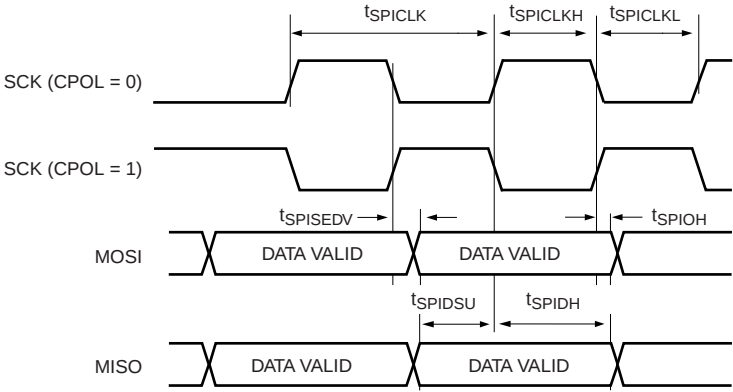
Fig 27. SPI master timing (CPHA = 0)
