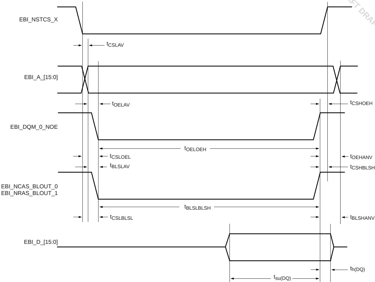
Fig 21. External memory read access to static memory
