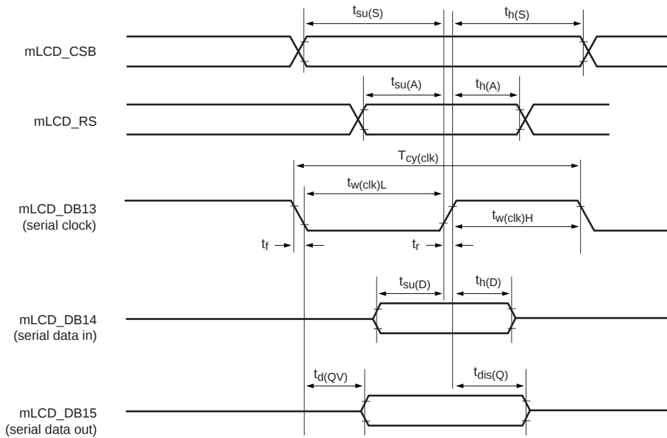
Fig 20. LCD timing (serial mode)
