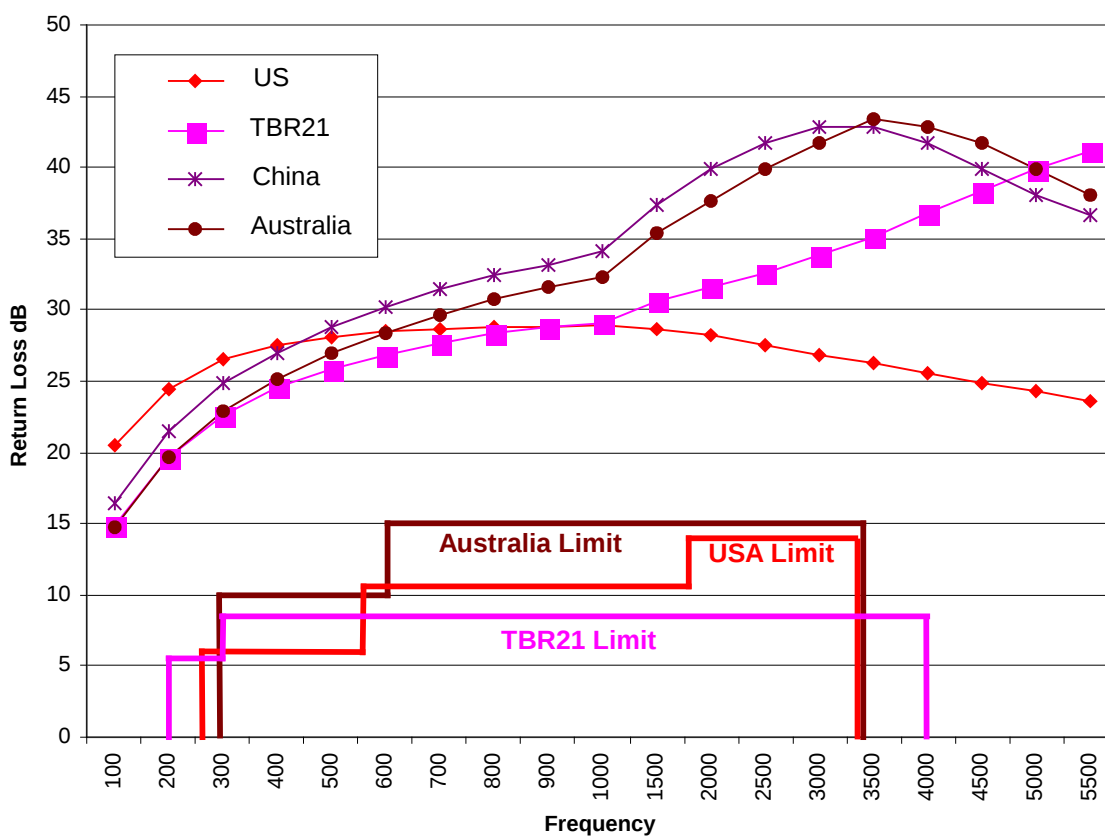
Figure 40: Return Loss
