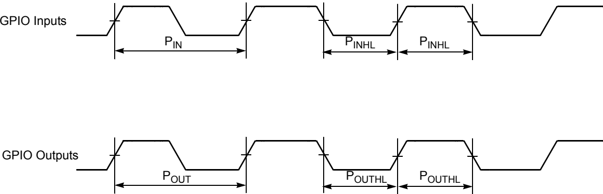
Figure 4-31 GPIO Timing
