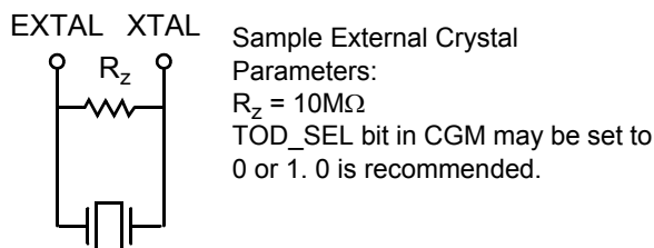
Figure 4-6 Crystal Oscillator
