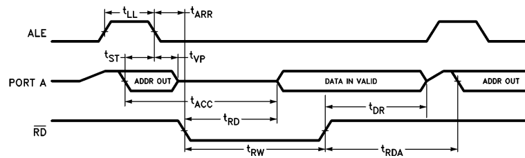
FIGURE 5. Read Cycle
