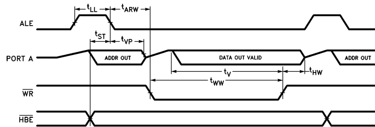
FIGURE 4. Write Cycle
