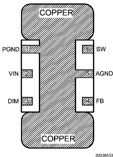
Thermal Design
