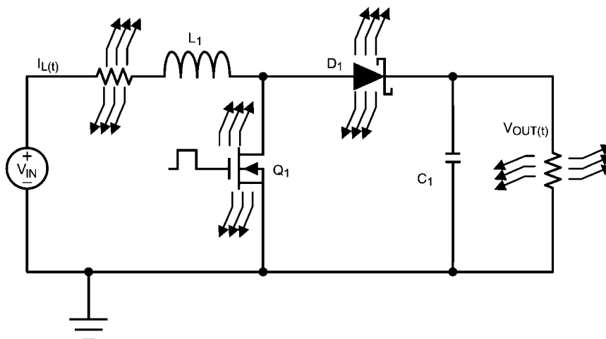
FIGURE 9. Thermal Schematic
