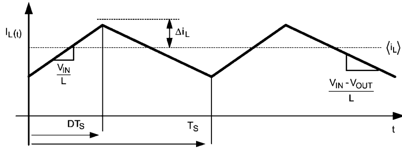
FIGURE 5. Inductor Current
