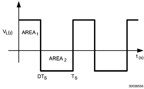
FIGURE 13. Inductor Volt-Sec Balance Waveform
