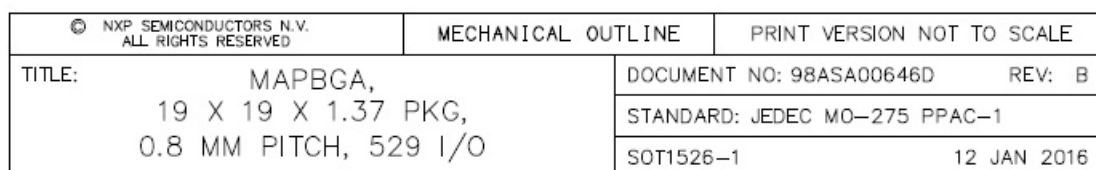
Figure 83. 19x19 mm BGA Package—Top, Bottom, and Side Views
