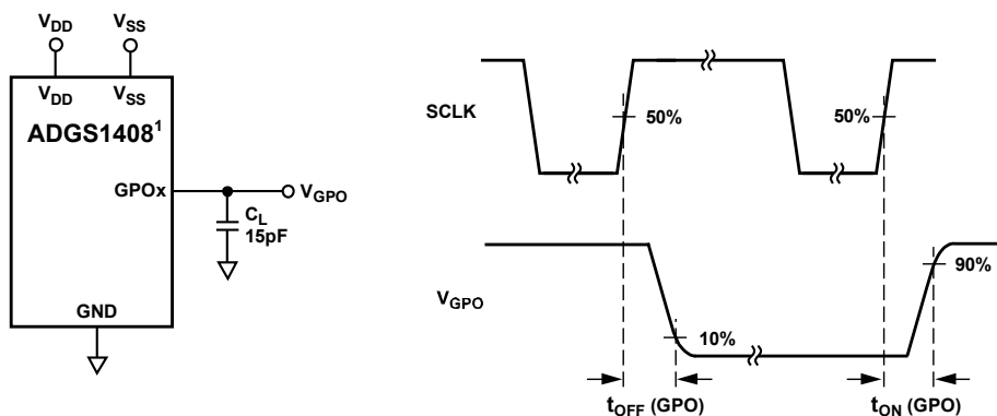
Figure 43. GPOx Timing, t ON (GPO) and t OFF (GPO)
