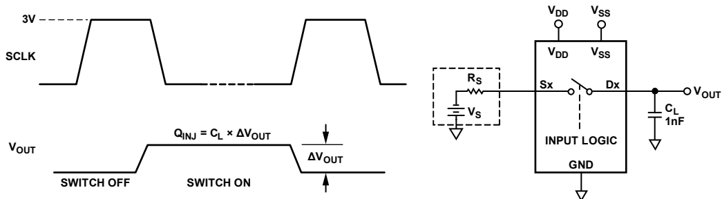
Figure 42. Charge Injection, Q_{\text{INJ}}
