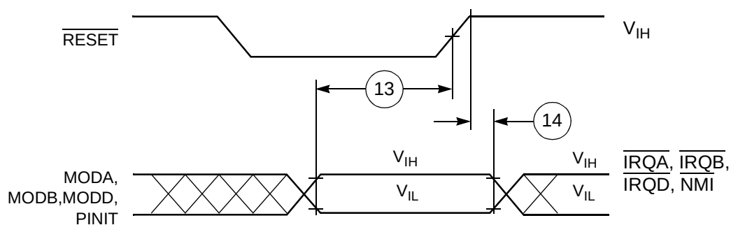
Figure 2-5. Operating Mode Select Timing
