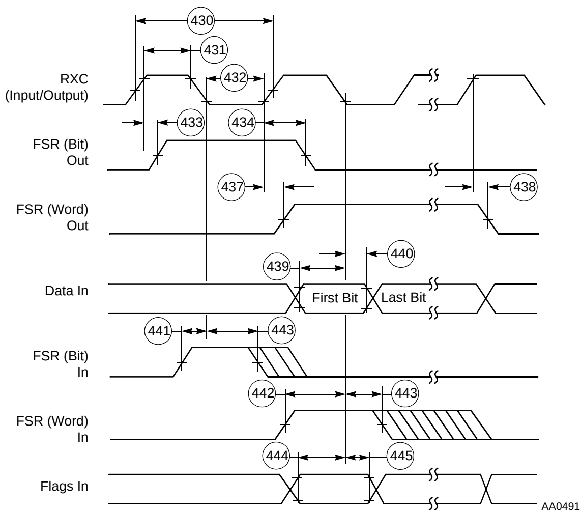
Figure 2-24. ESI Receiver Timing
