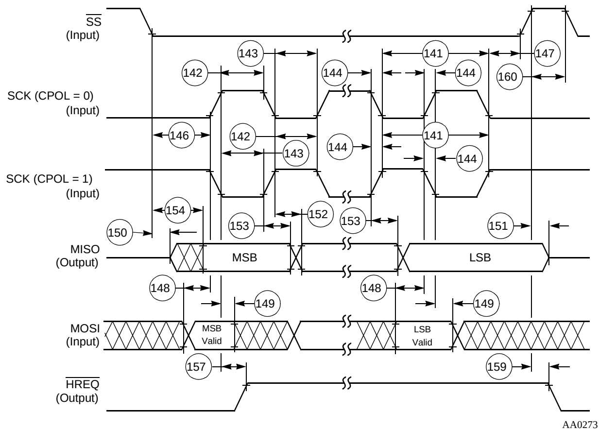
Figure 2-20. SPI Slave Timing (CPHA = 0)
