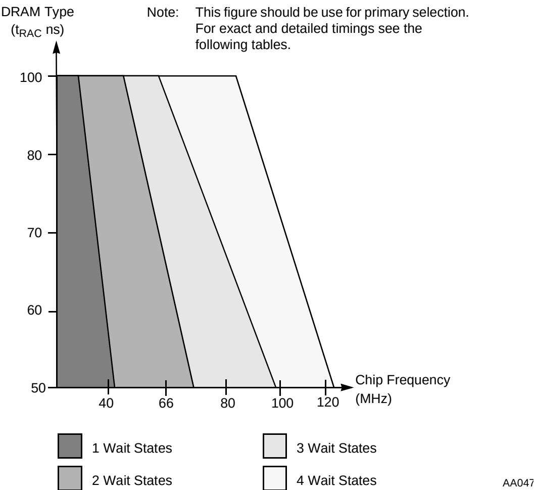
Figure 2-11. DRAM Page Mode Wait States Selection Guide
