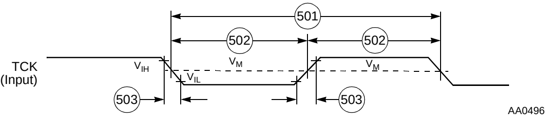
Figure 2-28. Test Clock Input Timing Diagram
