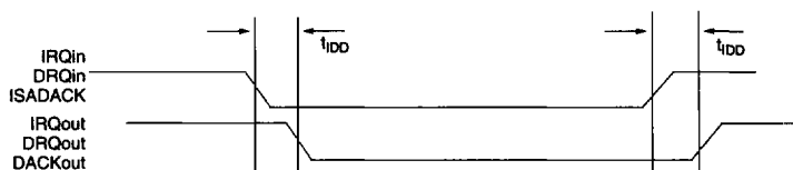
Propagation Delay for IRQ/DRQ/DACK
