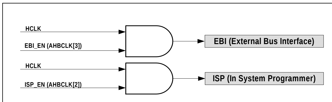
Figure 6-7 AHB Clock Source for HCLK
