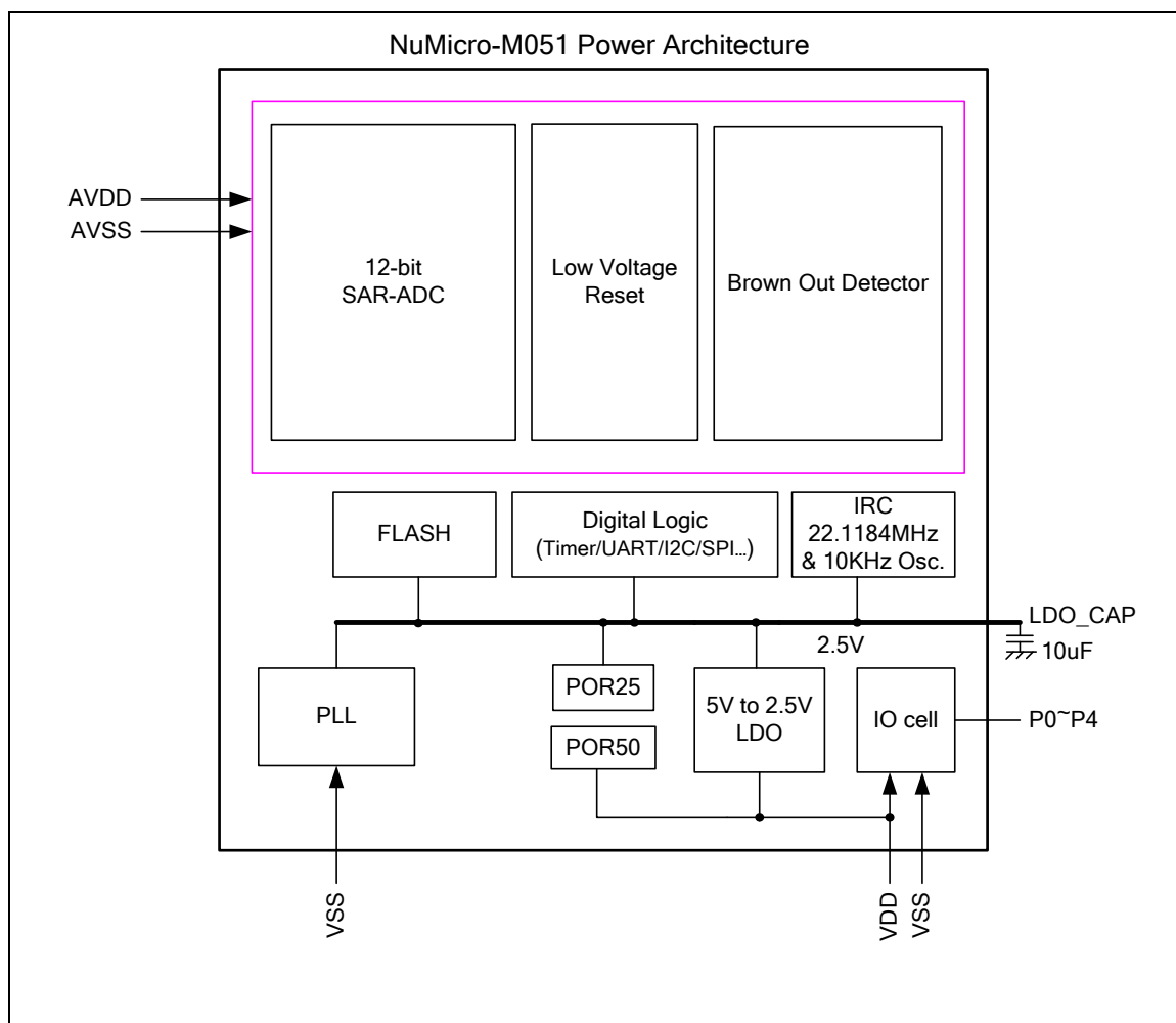
Figure 6-2 NuMicro M051™ Series Power Architecture Diagram
