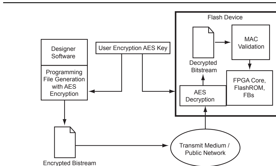
Figure 12-1 • AES-128 Security Features
