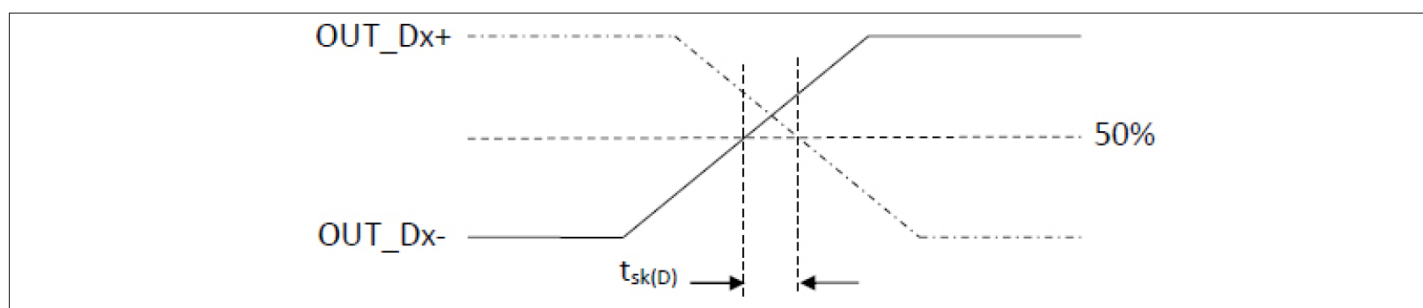
Figure 5-3 Intra-pair Skew( t_{sk(D)} ) Definition
