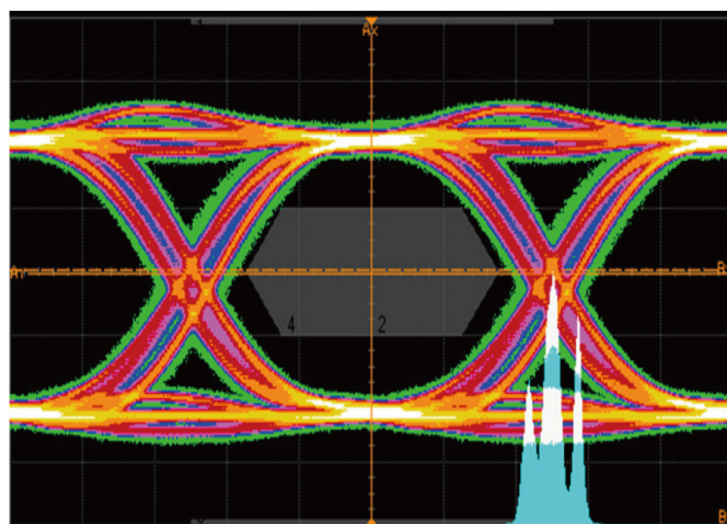
24" Input (-15.46dB loss) , EQ=2.5dB, 500mV Swing, Pre-emp =1.5dB, Rout_S0=1
