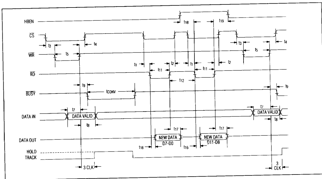
Figure 7b. Input/Output Port-Mode timing, two-byte read (MODE = 1).
