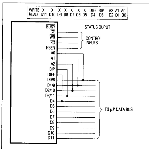
Figure 6. Input/Output Port Mode (12-Bit-Wide Data Bus Shown)
