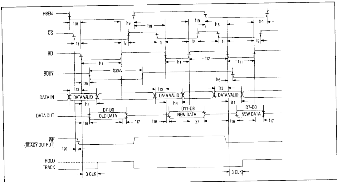
Figure 9b. ROM Mode timing, two-byte read (MODE = 0).
