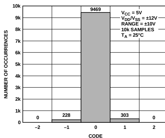
Figure 15. Histogram of Codes True Differential Mode
