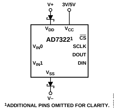
Figure 53. Schottky Diode Connection
