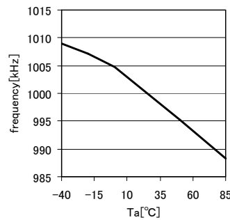
Fig.11 CH1 Switching Frequency Temperature Feature
