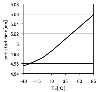
Fig.14 CH2,CH3 Soft Start Temperature Feature
