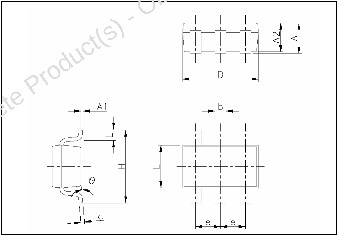
Figure 12. Package dimensions
