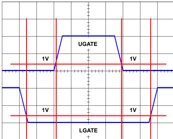
FIGURE 8. GATE DRIVER ADAPTIVE SHOOT-THROUGH
