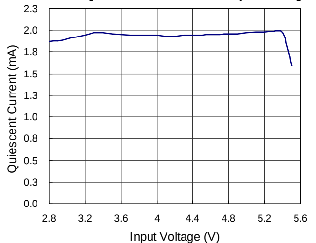
x1.5 Mode Quiescent Current vs. Input Voltage
