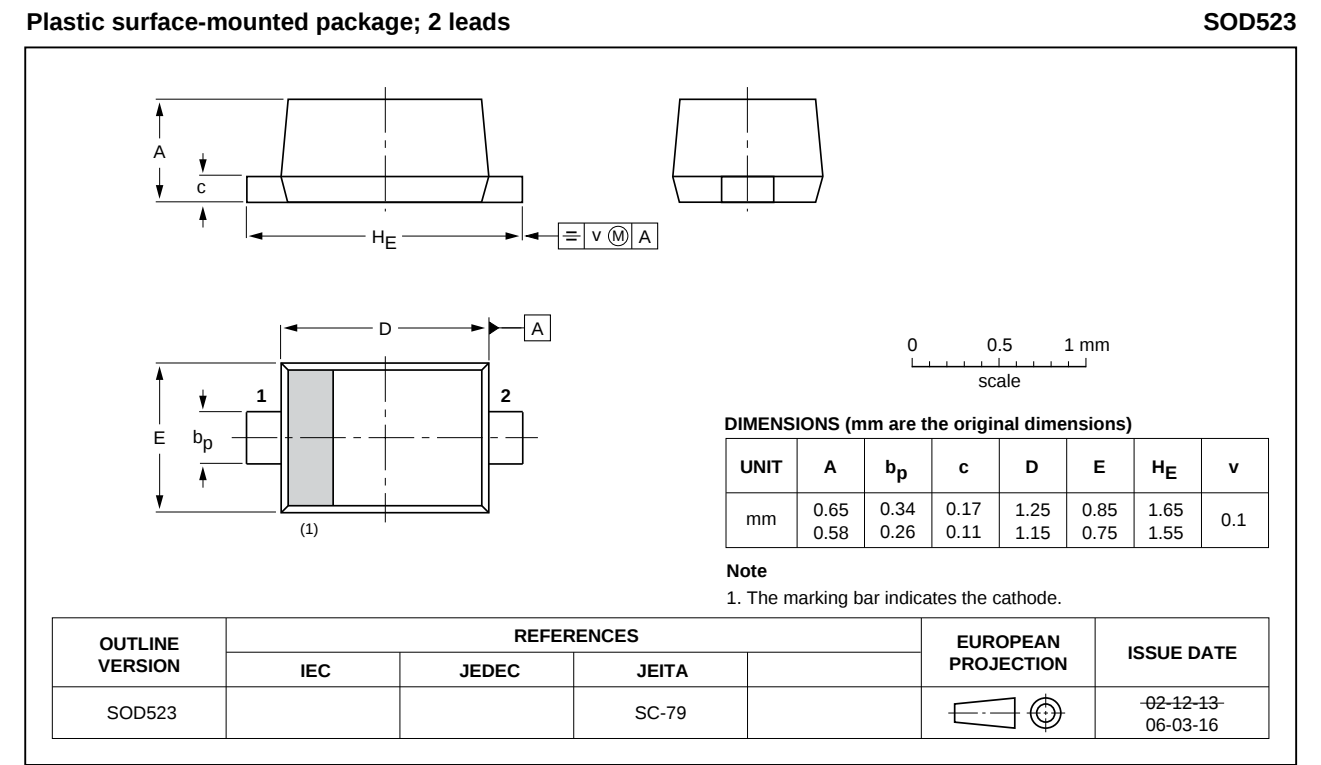
Fig 4. Package outline (BB208-02).
