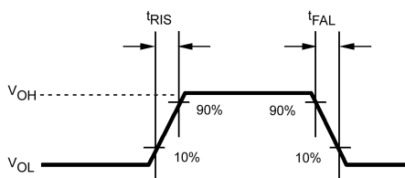
FIGURE 4. Rise and Fall Times
