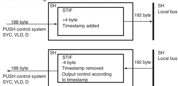
Schematic diagram of TS mode 1 and TS mode 2
