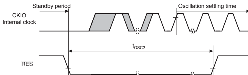
Figure 29.5 Power-On Oscillation Settling Time
