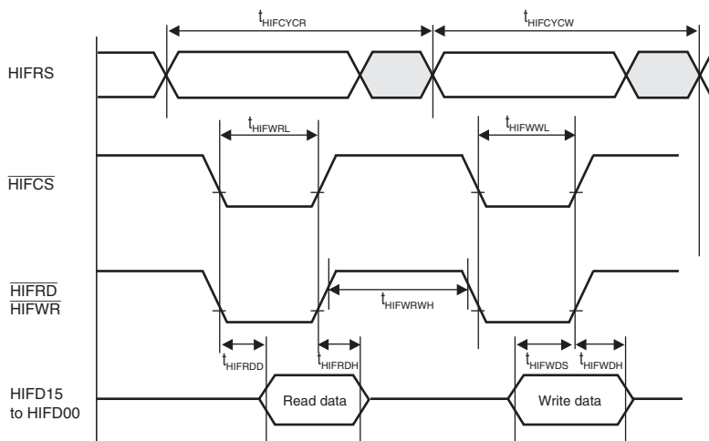
Figure 29.55 HIF Access Timing
