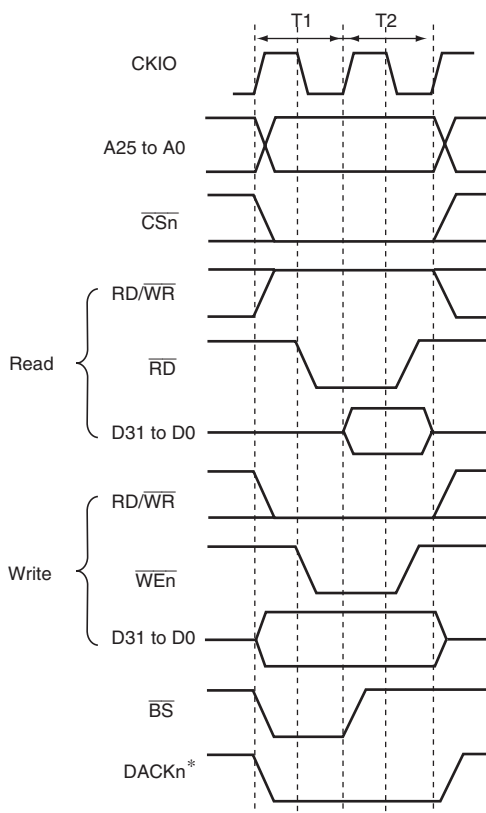
Figure 7.2 Normal Space Basic Access Timing (Access Wait 0)
