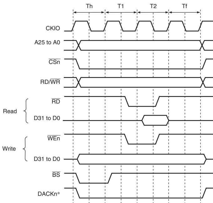
Figure 7.10 \overline{\text{CSn}} Assert Period Expansion
