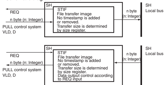
Schematic diagram of PS mode
