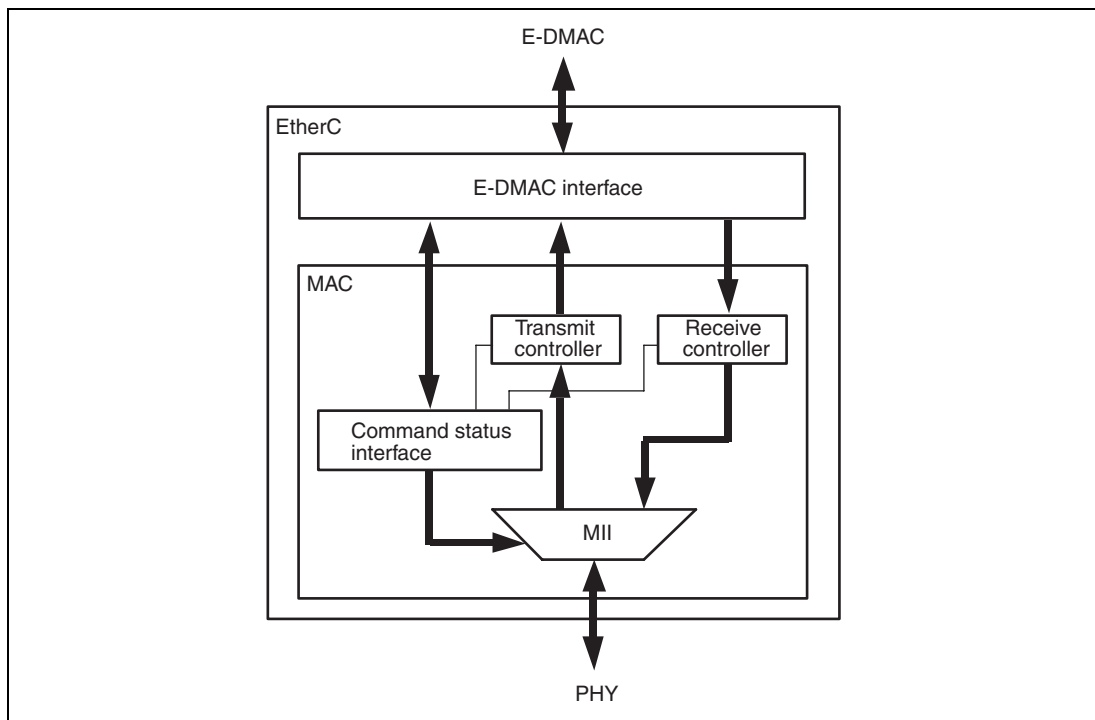
Figure 12.1 Configuration of EtherC
