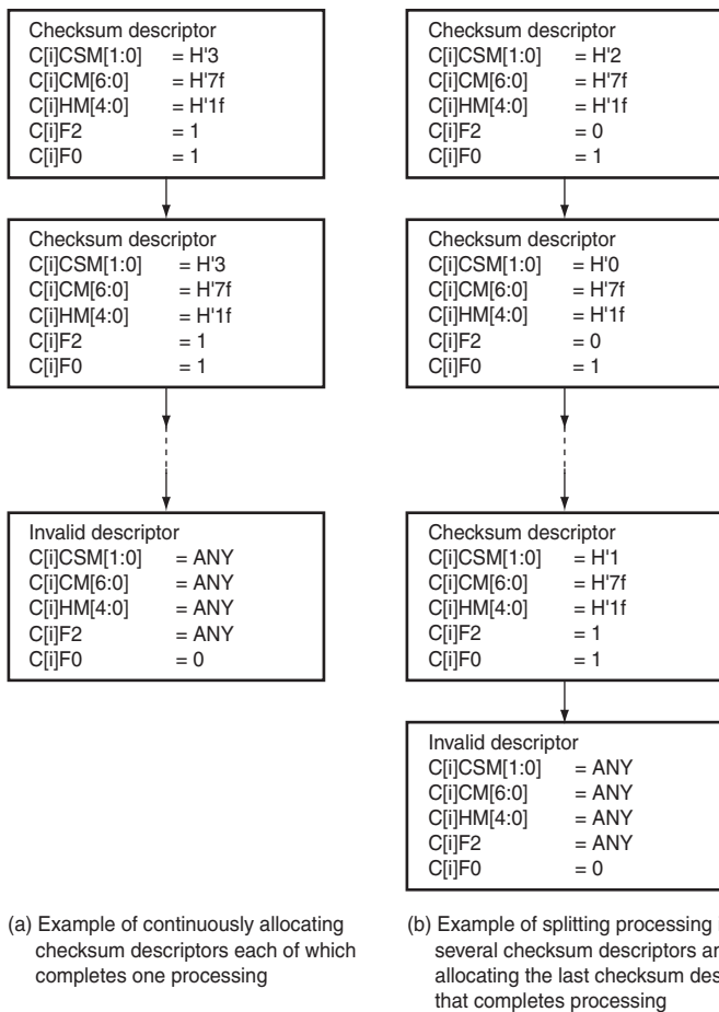
Figure 14.3 Examples of Allocating Checksum Descriptors
