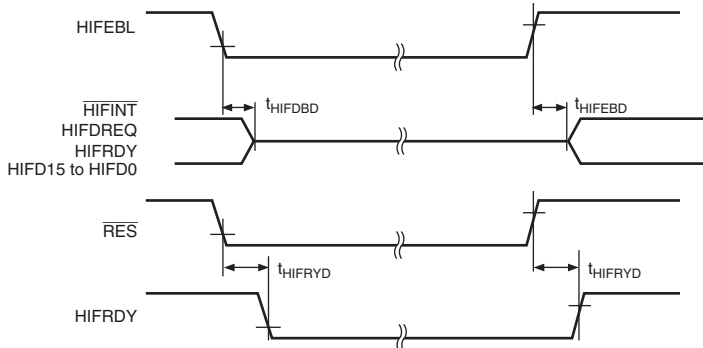
Figure 29.57 HIFRDY/HIF Pin Enable/Disable Timing
