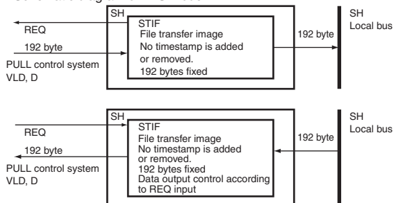
Schematic diagram of PS mode
