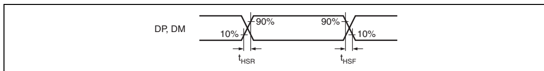
Figure 29.51 DP/DM Output Timing (for Low Speed)
