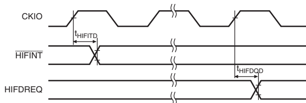
Figure 29.56 \overline{\text{HIFINT}} /HIFDREQ Timing
