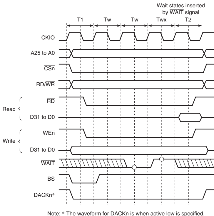
Figure 7.9 Wait Cycle Timing for Normal Space Access (Wait Cycle Insertion Using \overline{\text{WAIT}} Signal)
