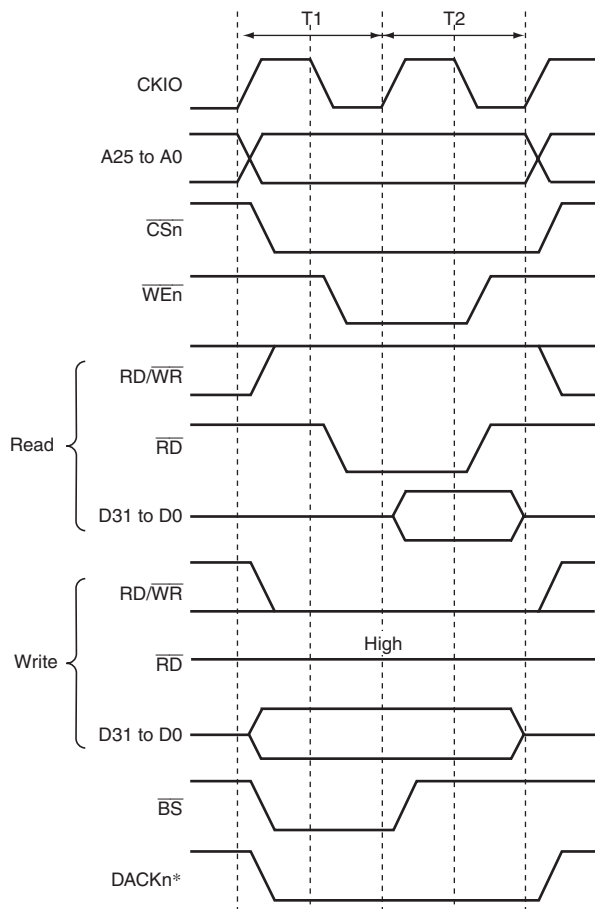
Figure 7.30 Basic Access Timing for SRAM with Byte Selection (BAS = 0)
