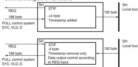
Schematic diagram of TS mode 3
