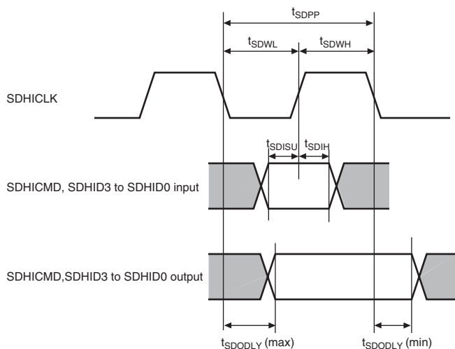
Figure 29.53 SD Card Interface
