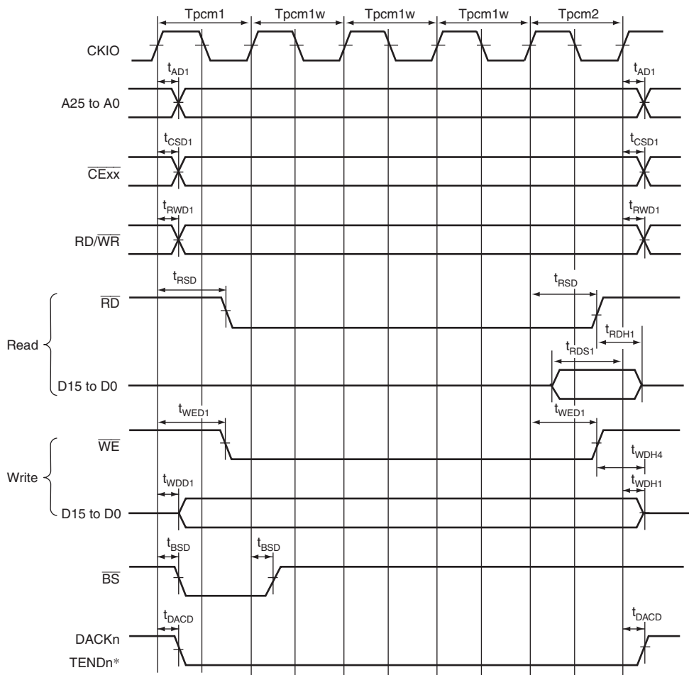
Figure 29.33 PCMCIA Memory Card Bus Cycle (TED = Zero Cycle, TEH = Zero Cycle, No Wait)
