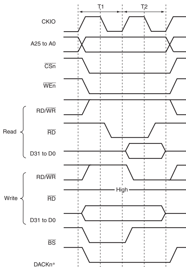
Figure 7.31 Basic Access Timing for SRAM with Byte Selection (BAS = 1)
