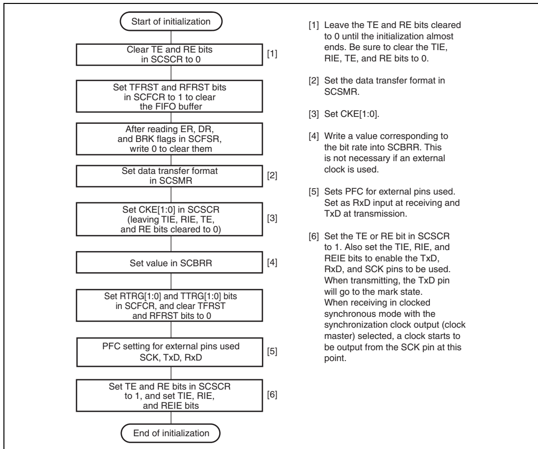
Figure 22.12 Sample Flowchart for SCIF Initialization
