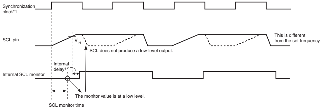
(c) When rising of SCL is gradual
