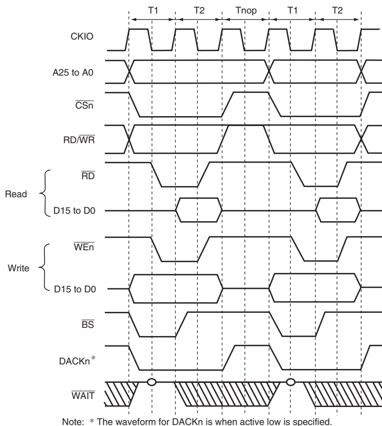
Figure 7.3 Continuous Access for Normal Space 1 Bus Width = 16 Bits, Longword Access, CSnWCR.WM Bit = 0 (Access Wait = 0, Cycle Wait = 0)
