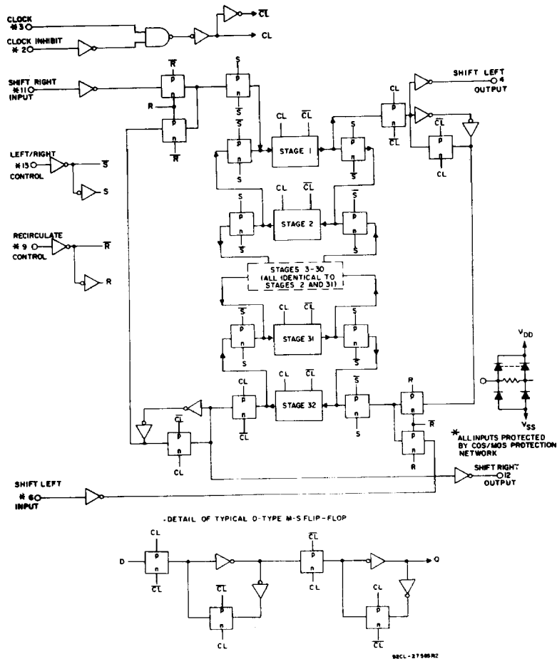
Fig. 3 - Logic diagram.
