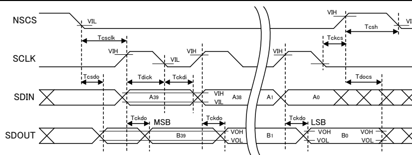
Fig.7.5 SPI Communication electrical characteristic
