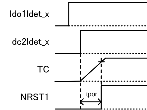
Fig.7.3 Power-on reset
