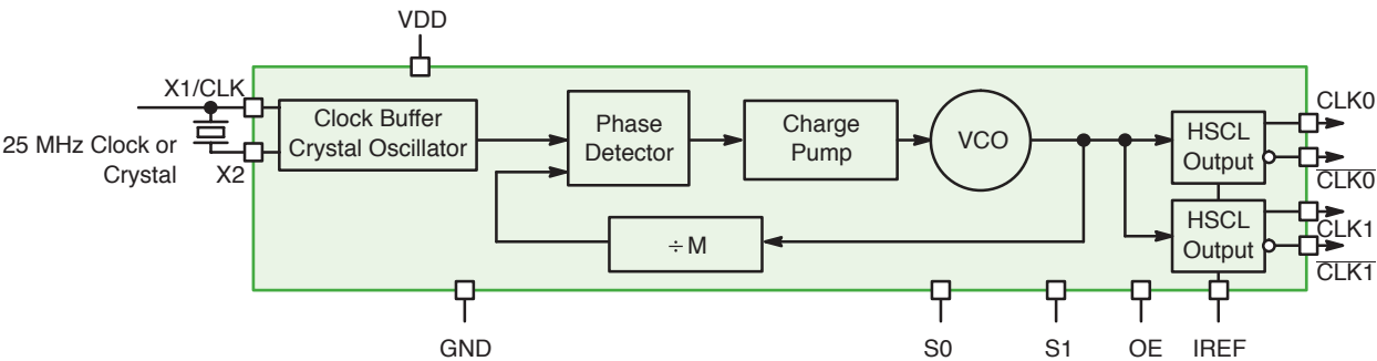
NB3N5573 Simplified Logic Diagram
