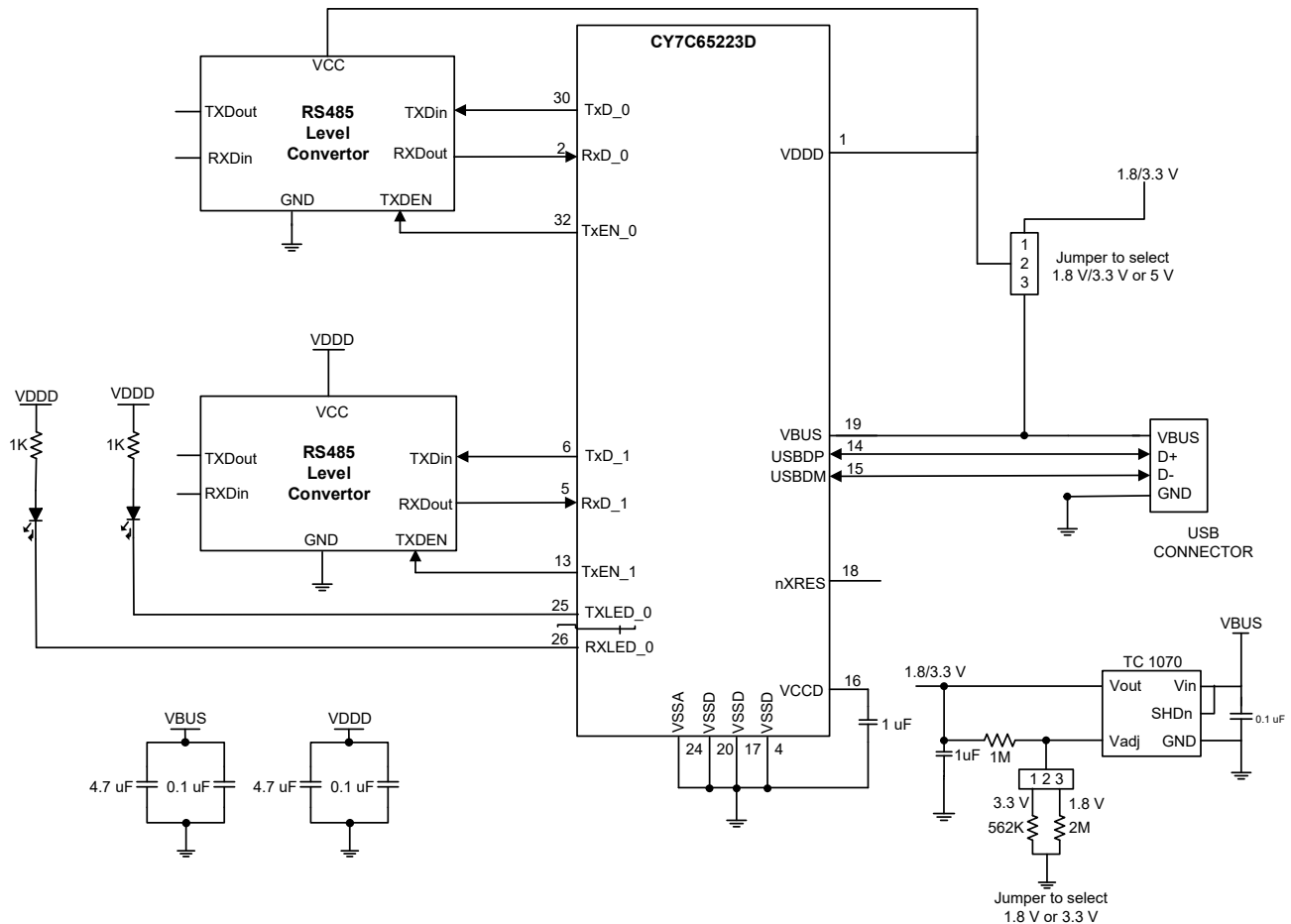
Figure 11. USB-to-RS485 Bridge
