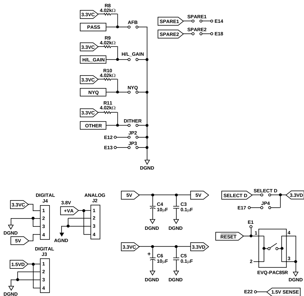
Figure 24. Evaluation Board
