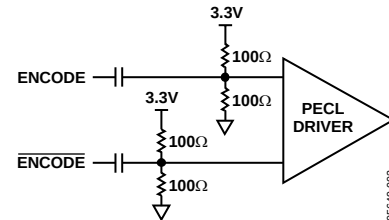
Figure 2. ENCODE Equivalent Circuit
