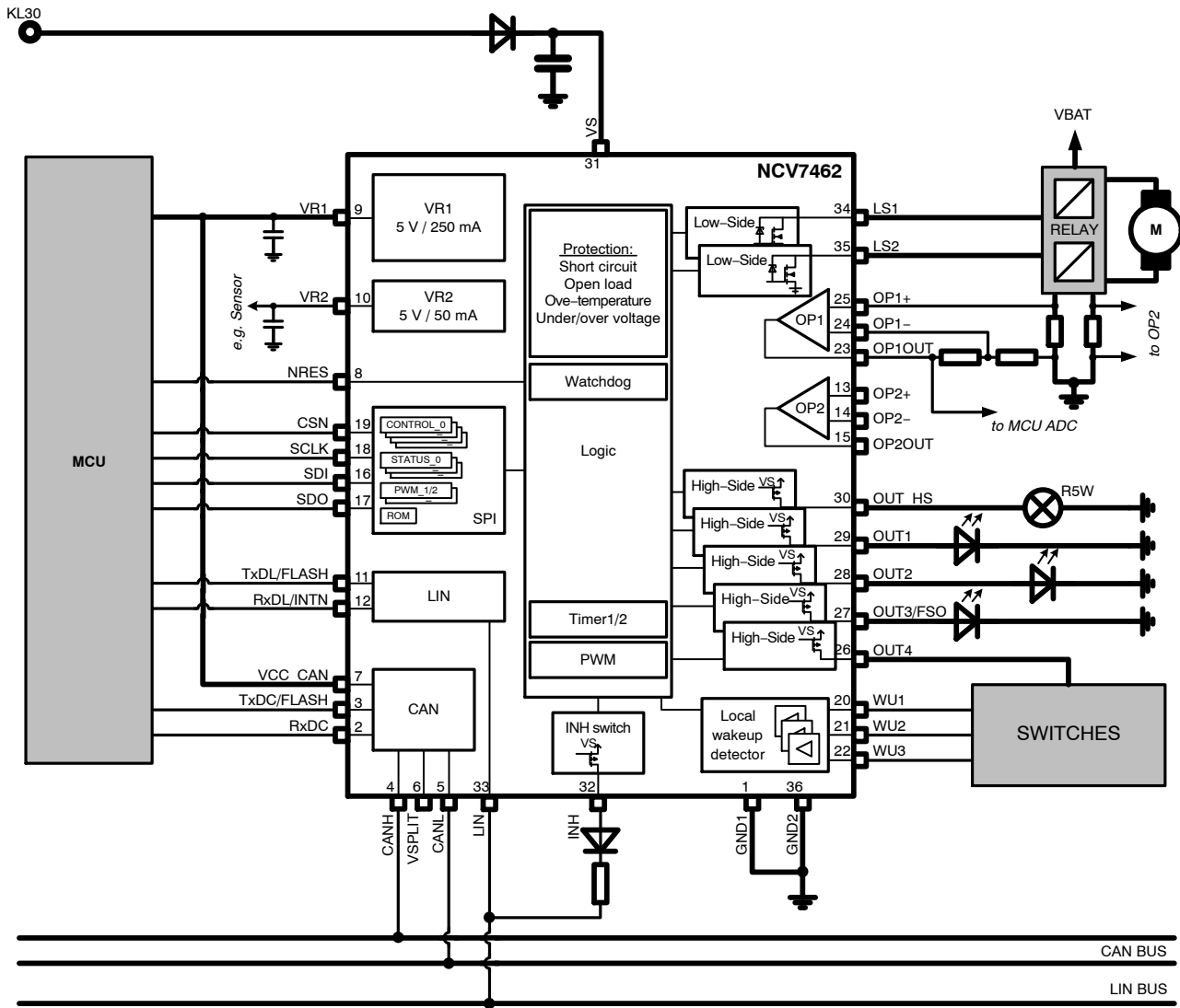
Figure 3. Application Diagram
