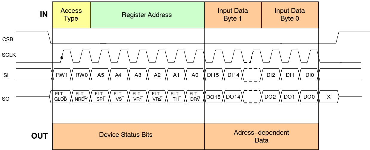
Figure 18. SPI Frame
