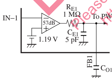
Figure 11. Error amplifier equivalent circuit
