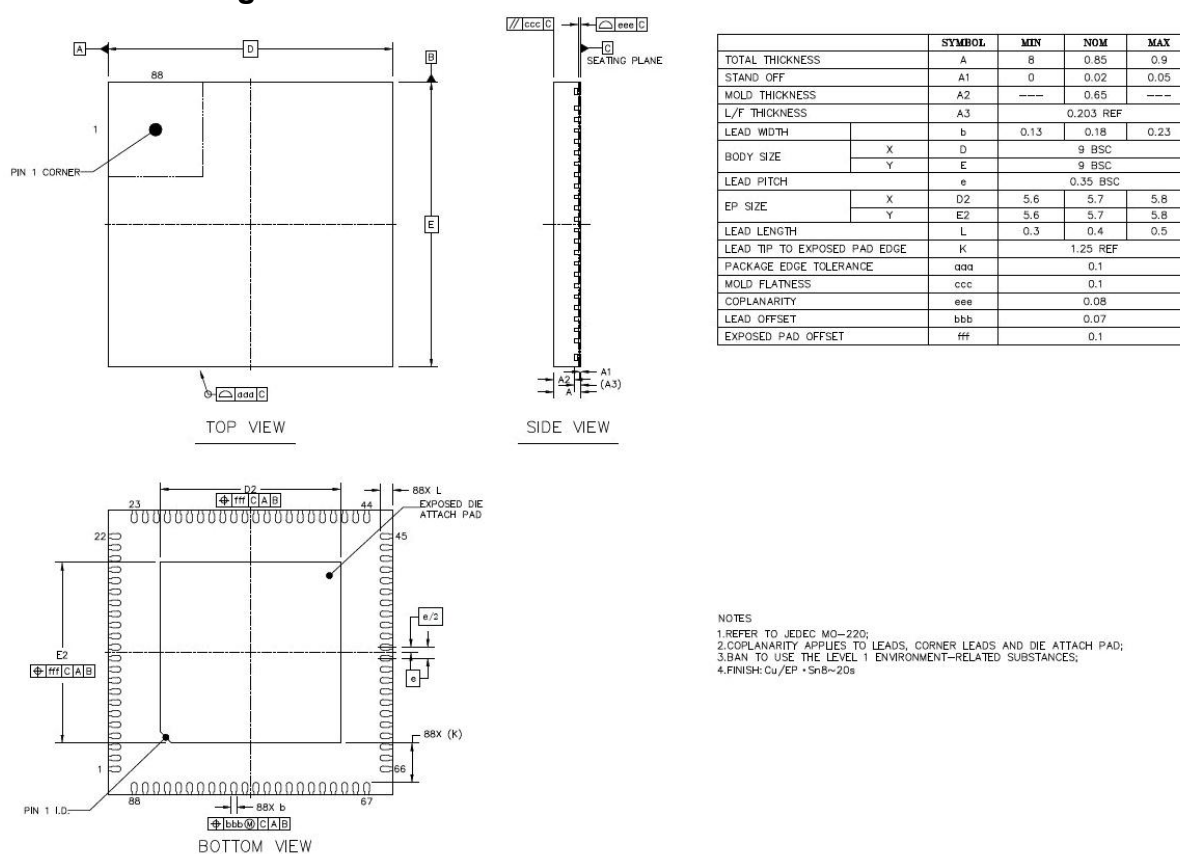
Figure 2-1 T31ZL package outline drawing
