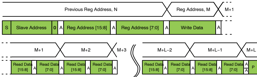
Figure 25. Sequential WRITE, Start from Current Location
