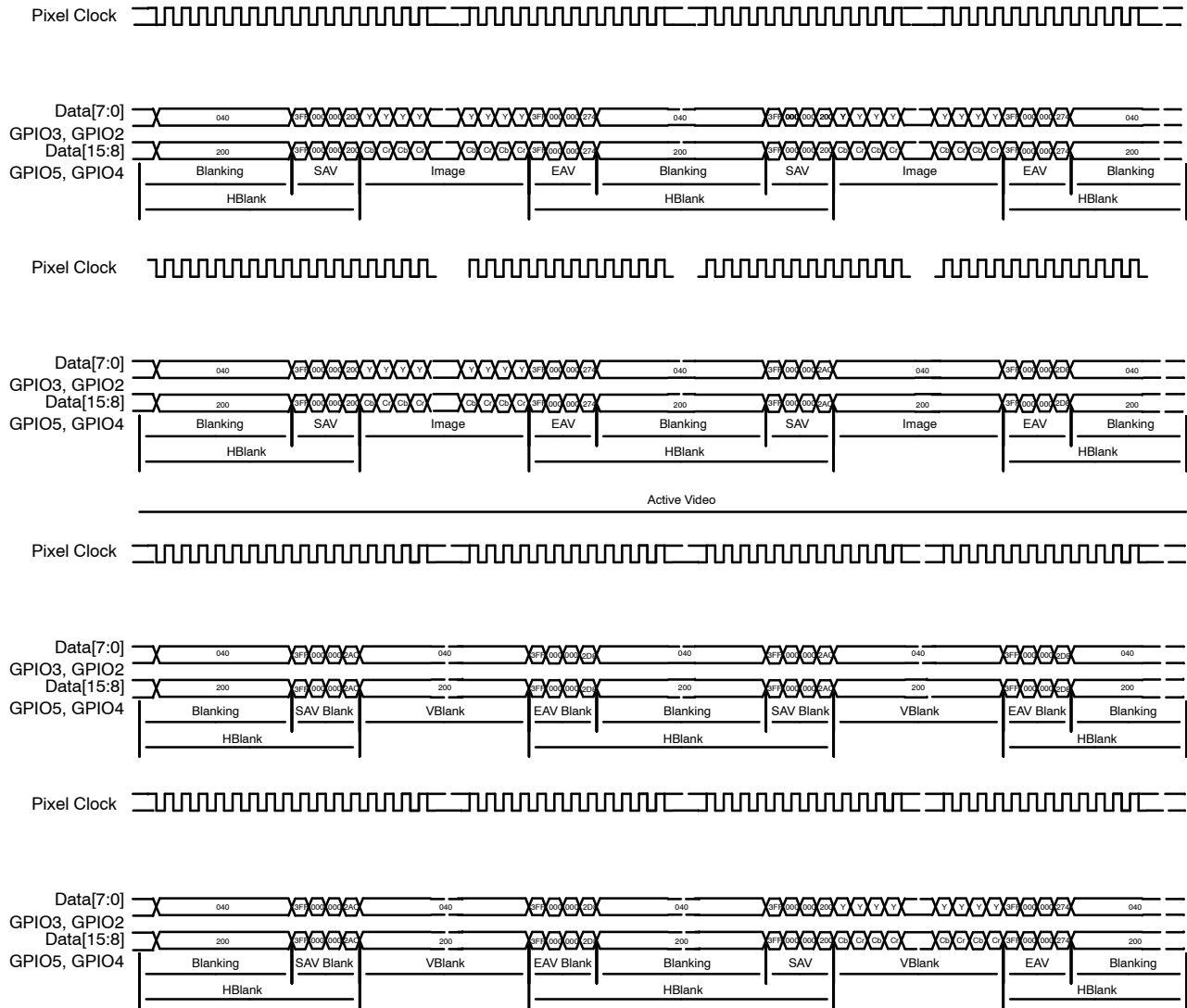
Figure 19. SMPTE296M Output
