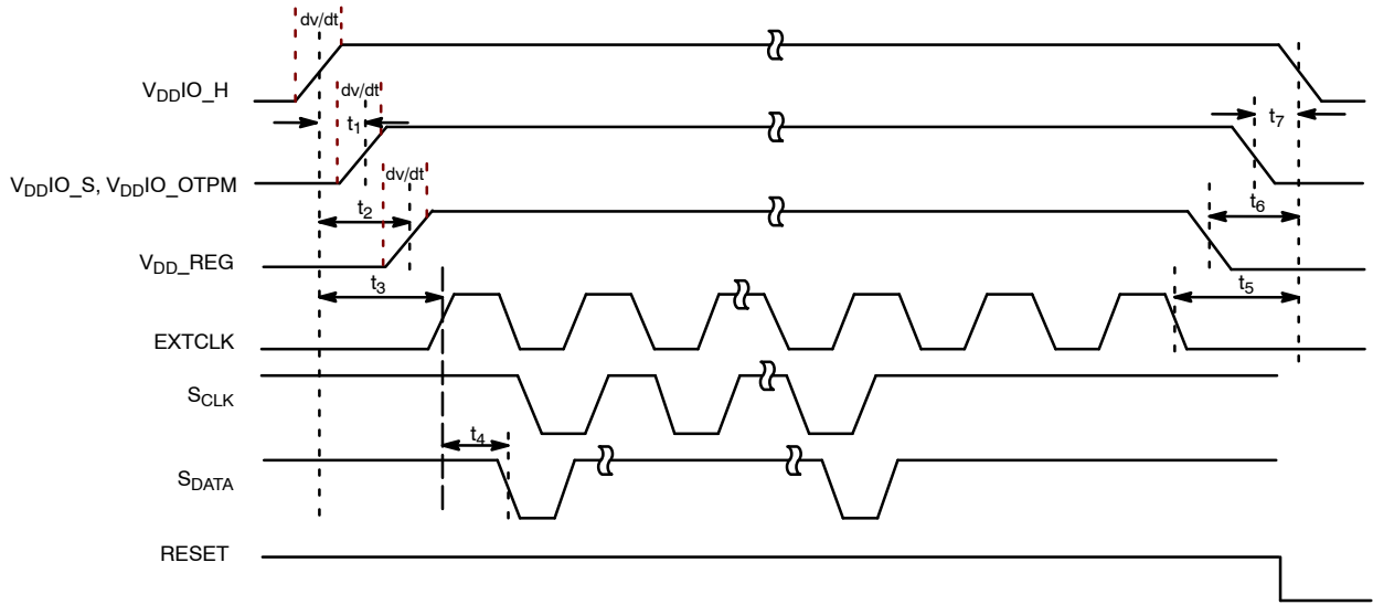
Figure 9. Power-Up and Power-Down Sequence
