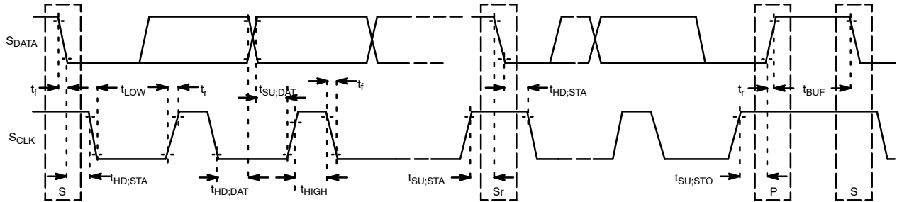
Figure 32. Master Two Wire Serial Bus Timing Parameters (CCIS)
