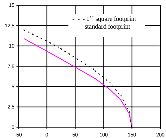
Figure 12 - Max. Cont. current (A) vs Amb. Temp. ( ^{\circ}C )
