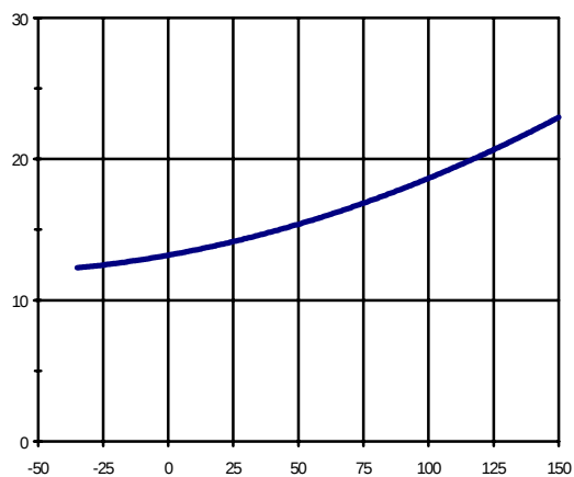
Figure 11 - R_{ds(on)} ( m\Omega ) vs T_j ( ^{\circ}C )
