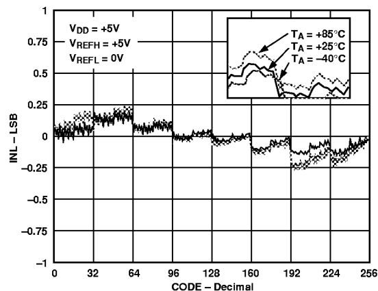
Figure 1. INL vs. Code
