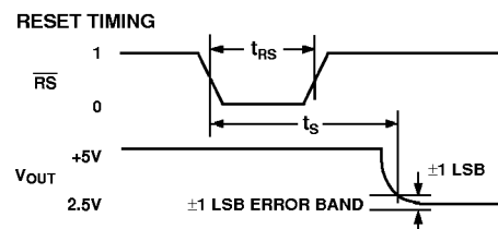
Figure 15c. Reset Timing Diagram
