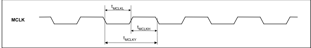
Figure 13 ADC and DAC Master Clock Timing Requirements
