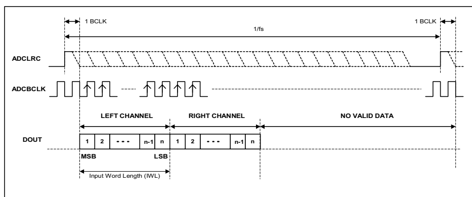
Figure 47 DSP Early Mode Timing Diagram – ADC Data Output
