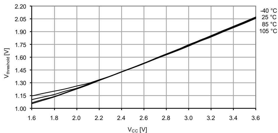
Figure 33-308. Reset Pin Input Threshold Voltage vs. V_{CC}
