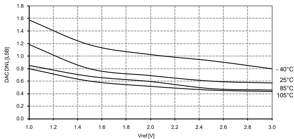
Figure 33-208. DAC DNL Error vs. V_{REF} V_{CC} = 3.6V
