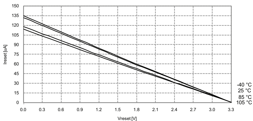
Figure 33-307. Reset Pin Pull-up Resistor Current vs. Reset Pin Voltage
