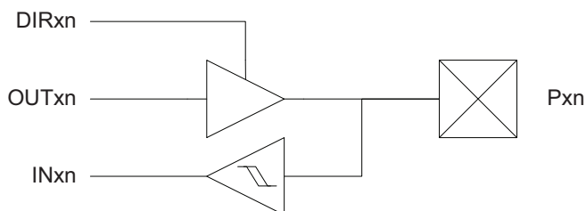
Figure 14-1. I/O Configuration - Totem-pole
