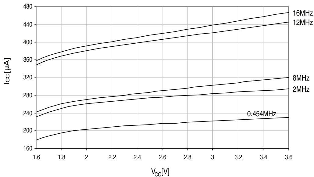
Figure 33-262. Standby Supply Current vs. V_{CC} T = 25^\circ\text{C} , running from different crystal oscillators
