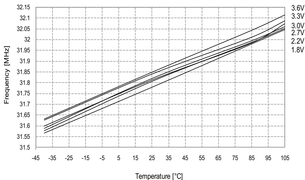
Figure 33-154. 48MHz Internal Oscillator Frequency vs. Temperature DPLL enabled, from the 32.768kHz internal oscillator
